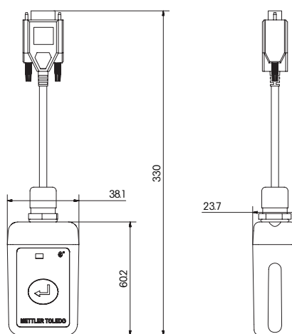
ACM360-D1 9 D-Sub female version (general application)
